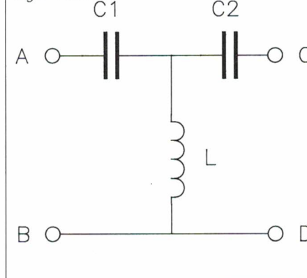
Fig 2 T-filter
