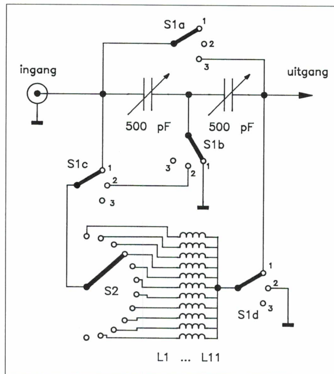
Fig 3 Schema tuner
