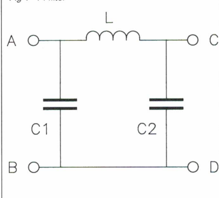
Fig 1 Pi-filter
